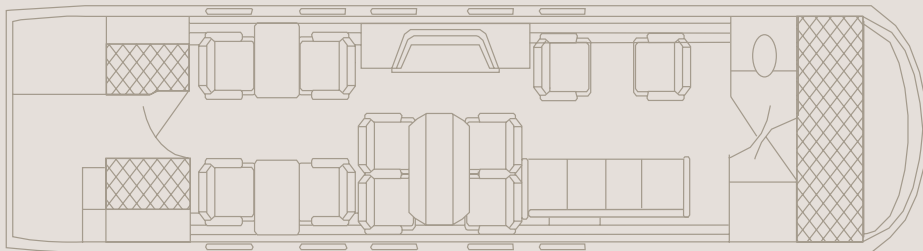
GULFSTREAM III CABIN CONFIGURATION
